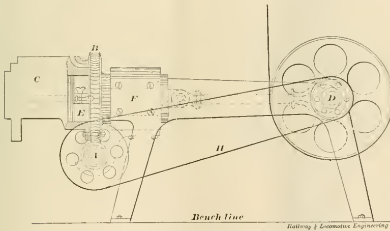
SKETCH OF TRIPLE PISTON RING GRINDING MACHINE.
